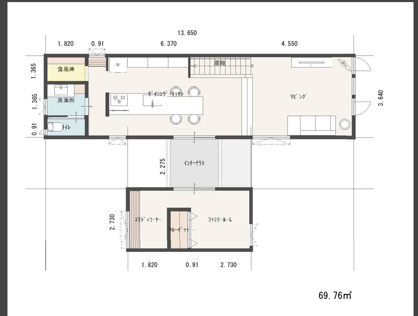
PLAN VIEW 2F
